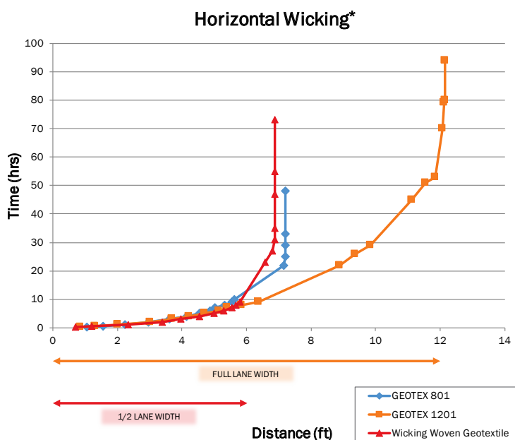
Figure 8 - geotextile horizontal wicking - distance vs time -- Testing based on ASTM C1559
