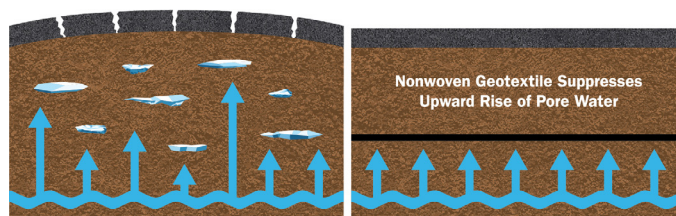
Figure 10 - Function of a capillary break
