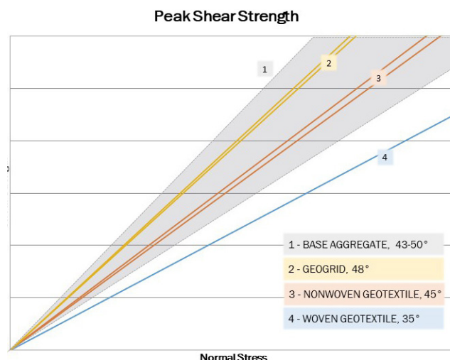
Figure 11 - Geosynthetic interface friction relative to road base aggregate
