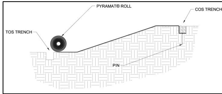
Figure 6: Placement of PYRAMAT across Slope
